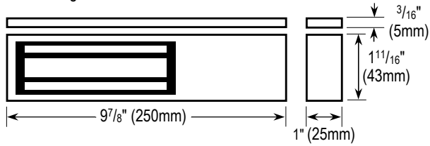
Electromagnet
